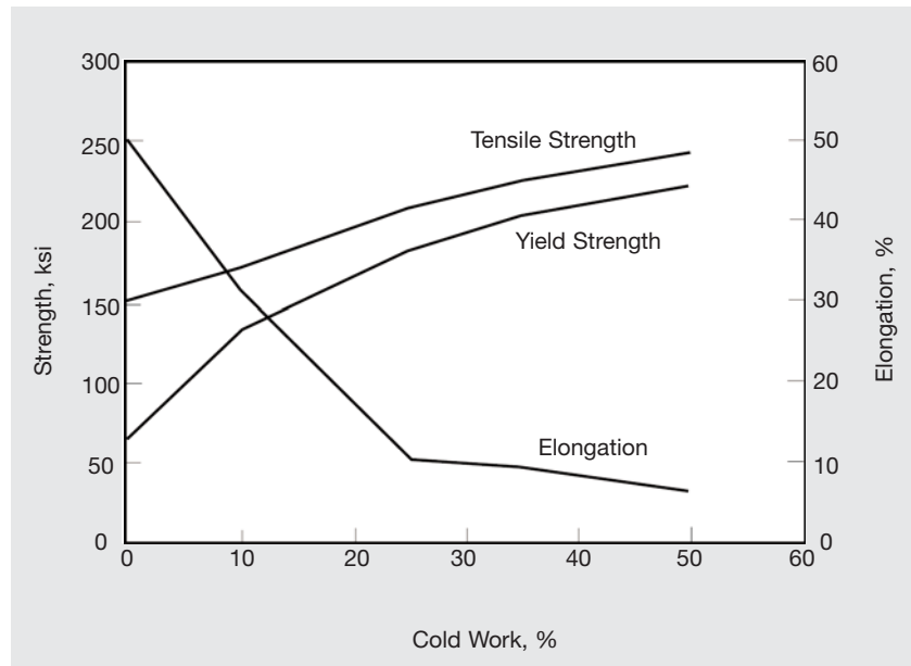
Figure 2 - Effect of cold work on mechanical properties of UDIMET alloy 188.
