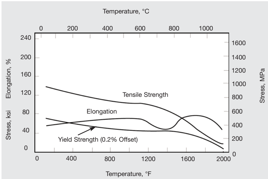
Figure 1 - Tensile strength, elongation and yield strength of UDIMET alloy 188.
