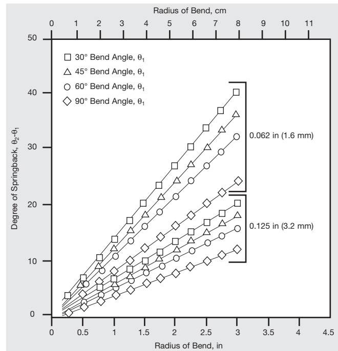
Figure 8. Degree of springback for INCONEL alloy 625LCF. Nominal gauge is 0.062 in (1.6 mm) and 0.125 in (3.2 mm) at 60 ksi (414 MPa) yield strength.
