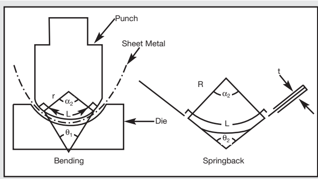
Figure 7. Schematic defining bend angle, bending radius and thickness used in equation 6.
