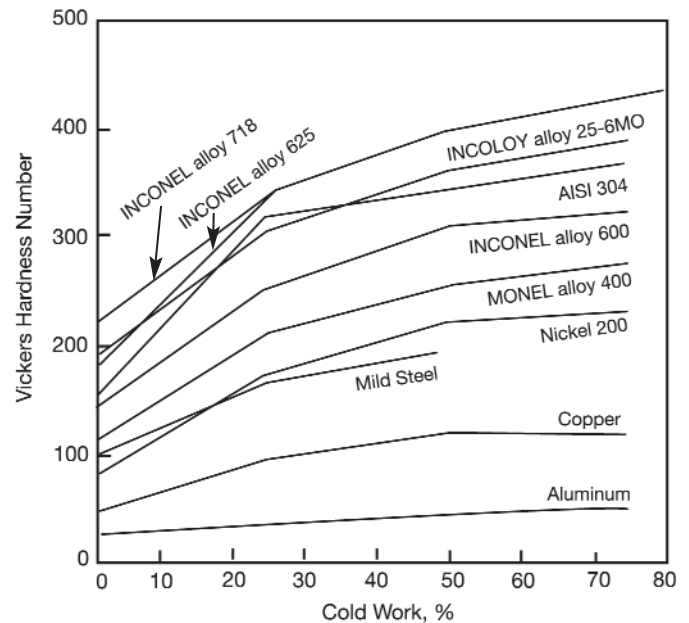
Figure 6 - The work-hardening rate for INCOLOY alloy 25-6MO is similar to that for AISI 304 stainless steel.
