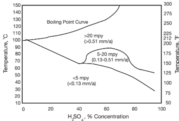
Figure 4 - Isocorrosion chart for INCOLOY alloy 25-6MO in sulfuric acid.
