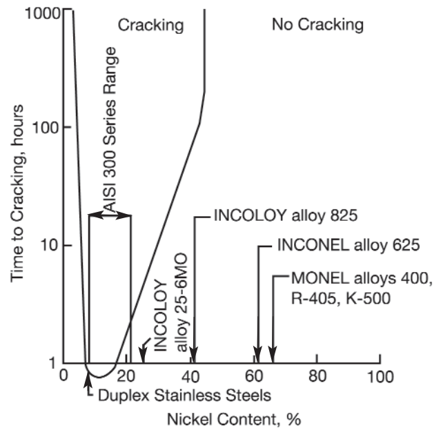
Figure 3 - The Copson U-Curve. The classic indicator of susceptibility to chloride-ion stress-corrosion cracking is the boiling 42% magnesium chloride test. INCOLOY alloy 25-6MO, with 25% nickel and an addition of nitrogen which acts synergistically with the nickel, offers significantly better resistance to chloride-ion stress-corrosion cracking than the lower nickel content stainless steels, such as AISI 317.
