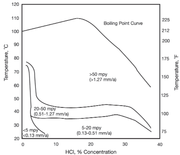
Figure 5 - Isocorrosion chart for INCOLOY alloy 25-6MO in hydrochloric acid.
