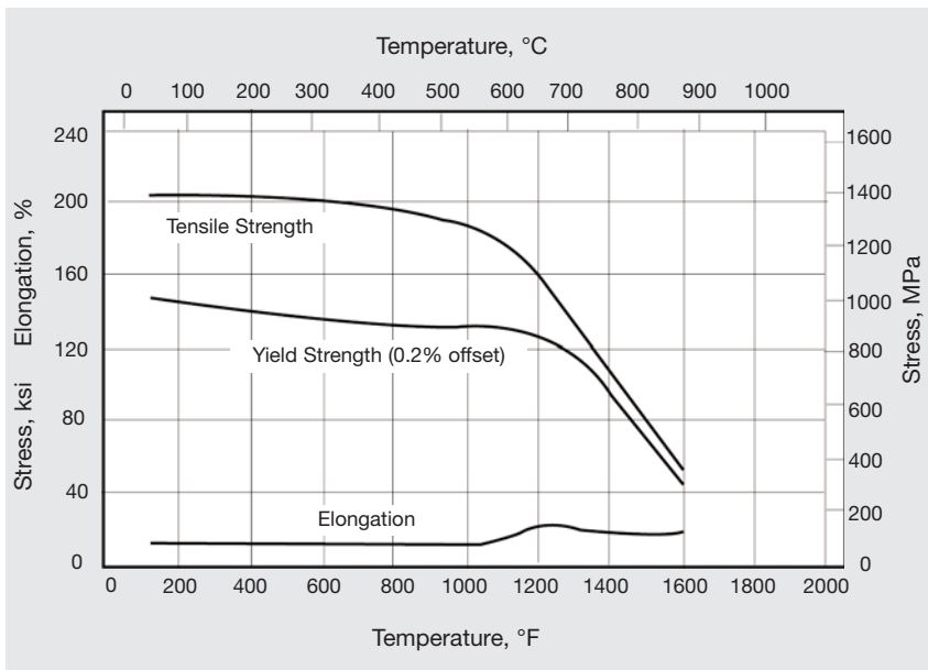
Figure 1. Typical mechanical properties of precipitation-hardened UDIMET alloy D-979
