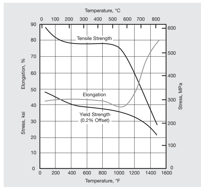
Figure 2. High-temperature tensile properties of INCOLOY alloy 800 hot-rolled rod.
