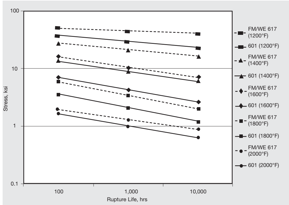
Figure 17. Rupture Strength Comparison. INCONEL alloy 617 Welding Products vs. INCONEL alloy 601 Wrought Products.
