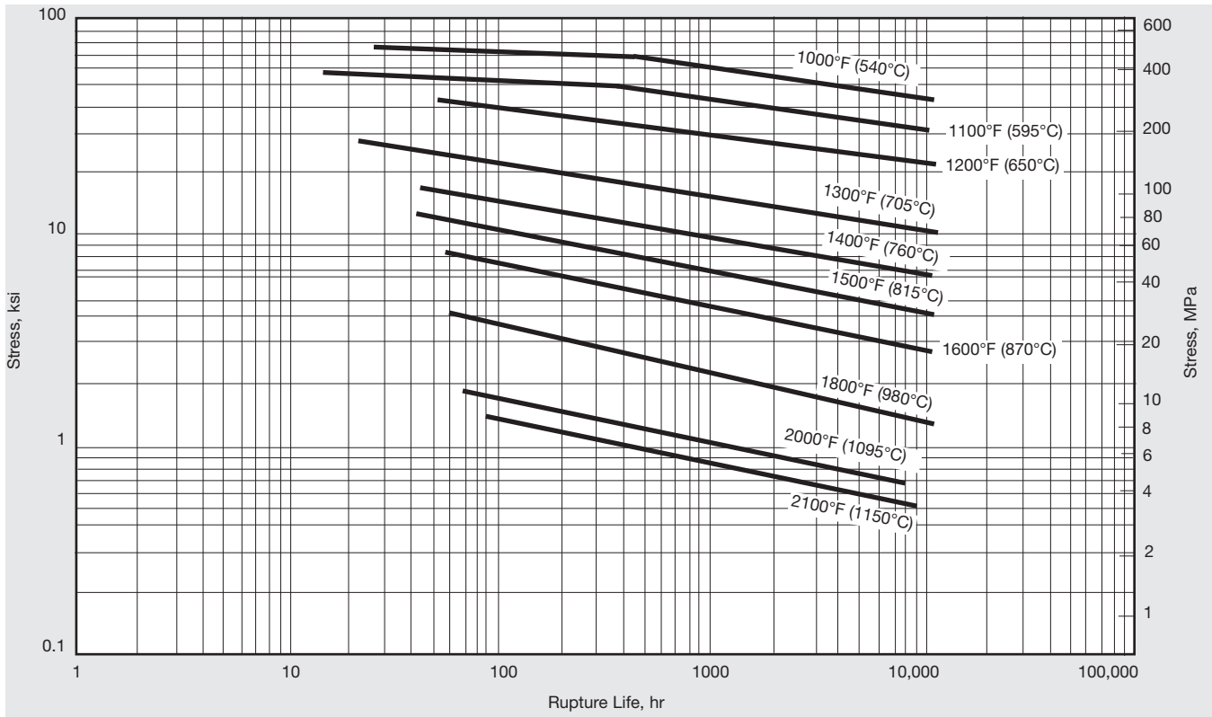
Figure 7. Typical rupture strength of solution-treated (2100°F) (1150°C) INCONEL alloy 601.
