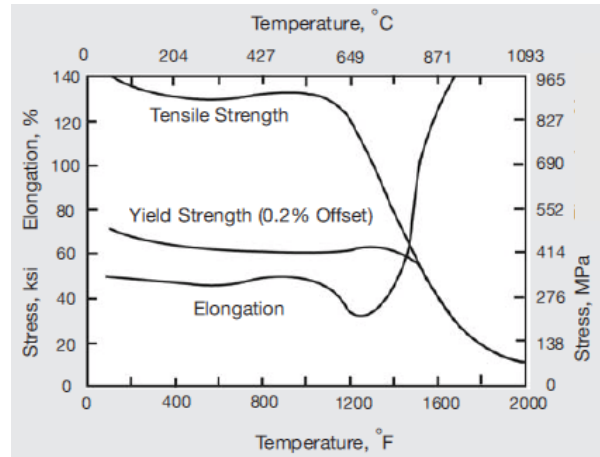
Figure 3 – High-temperature tensile properties of annealed bar.
