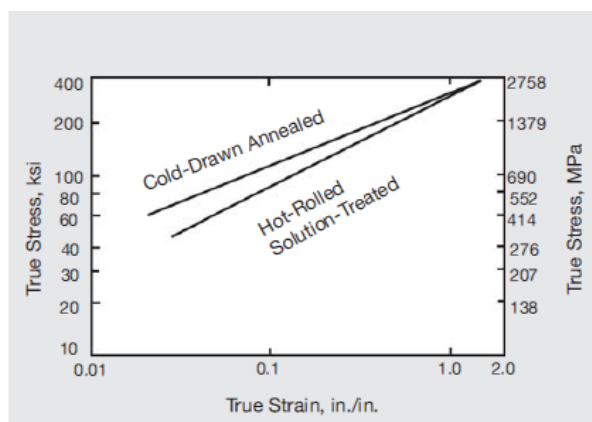
Figure 2 – True stress-true strain of round.
