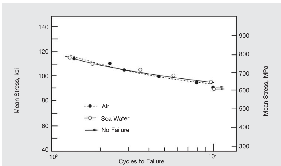
Figure 4 - Mean axial stress vs. cycles of fatigue for INCONEL alloy 725 in the dual aged condition [1350°F (732°C)/8h, FC@100°/h., 1150°F (621°C)/8h/AC] tension-tension test. Tested at the LaQue Center for Corrosion Technology. (R-value = Min. stress/Max. Stress=0.6)
