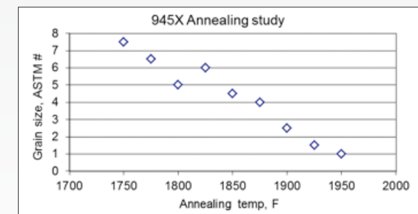
Figure 14: Grain size versus annealing temperature of alloy 945X®
