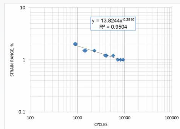
Figure 4: Strain controlled low cycle fatigue (LCF) tested at 450°F [232°C] as per ASTM E606-4. Tests were done using sinusoidal waveform at a frequency of 10 CPM. R-ratio for all was -1.
