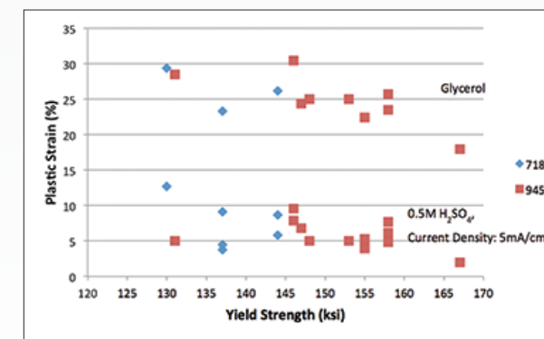
Figure 9 shows plastic strains of alloy 945X ® and 718 in glycerol and in the listed environment.
