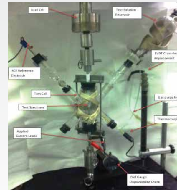
Figure 8: A specially designed apparatus used to evaluate hydrogen embrittlement resistance.
