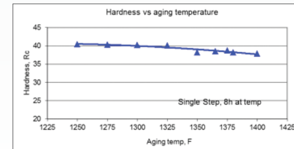
Figure 15: Hardness of alloy 945X® on single step age hardening in the temperature range of 1250 to 1400F.
