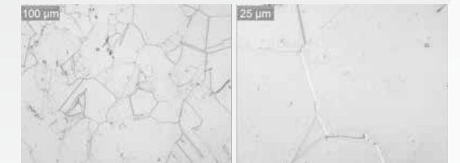
Figure 16: Optical photographs of 22-inch [560 mm] diameter rod of alloy 945X® at center in longitudinal orientation.
