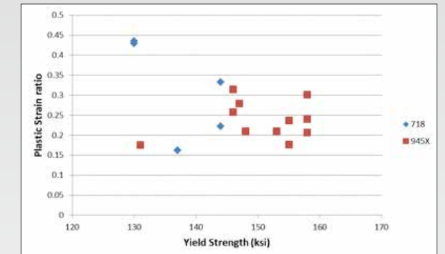
Figure 10 shows plastic strain ratios of alloy 945X ® and 718 in glycerol and in the listed hydrogen embrittlement environment. The latter is divided by the former to get these values.
