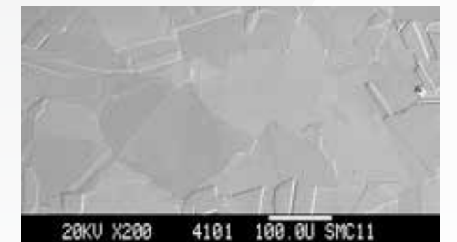
Figure 17: Scanning electron micrographs of 10-inch [254 mm] diameter alloy 945X® rod at center in longitudinal orientation.
