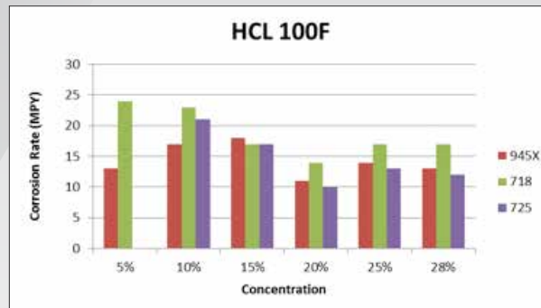
Figure 11: Weight loss of alloys 945X®, 718 and 725 at various HCl concentrations 100°F [38°C]
