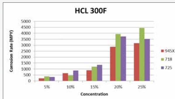
Figure 13: Weight loss of alloys 945X®, 718 and 725 at various HCl concentrations 300°F [149°C]
