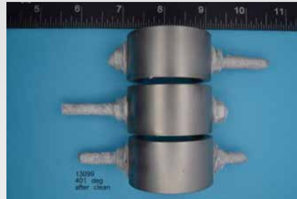
Figure 5: Photograph of a set of C-rings after 90 days exposure in 180,000 mg/L Cl, 500 psi [3.5 MPa] H 2 S and 500 psi [3.5 MPa] CO 2 at 401°F [205°C]
