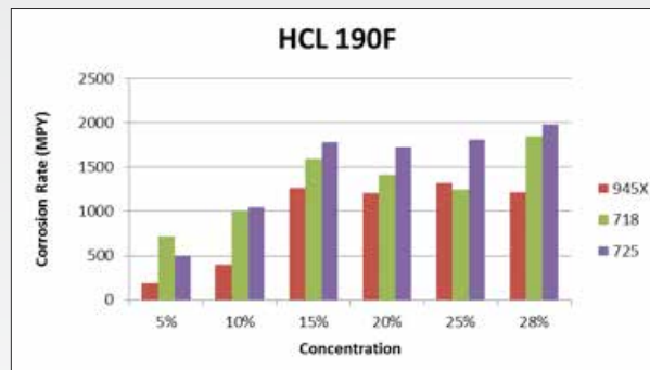
Figure 12: Weight loss of alloys 945X®, 718 and 725 at various HCl concentrations at 190°F [88°C]
