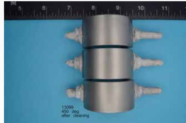
Figure 6: Photograph of a set of C-rings after 90 days exposure in 139,000 mg/L Cl, 500 psi [3.5 MPa] H 2 S and 500 psi [3.5 MPa] CO 2 at 450°F [232°C]
